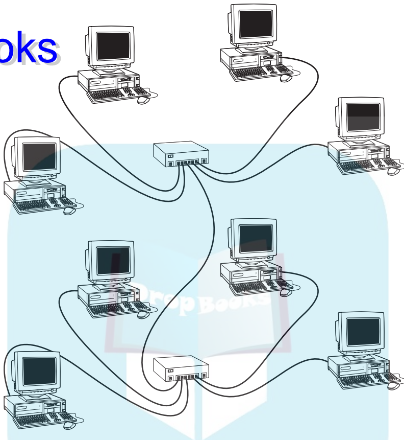
Figure 5-5: You can daisy-chain hubs or switches together.
